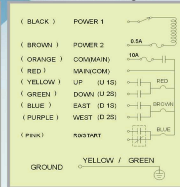
F21-4S/4SB/2D Wire Diagram
