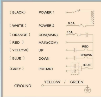
F21-2S Wire Diagram
