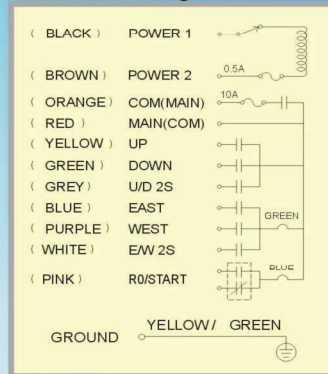
F21-4D Wire Diagram
