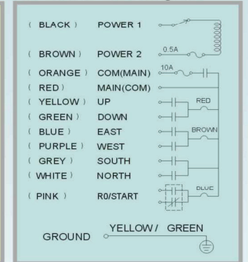
F21-E1/E1B Wire Diagram
